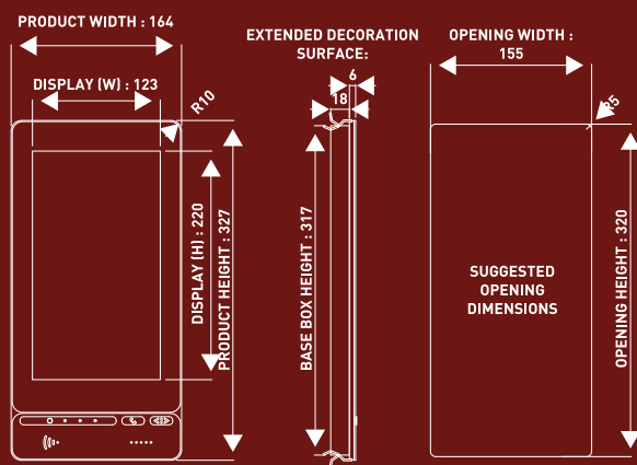
10.1" COP Dimensions: 164mm W x 327mm H x 24 mm D
